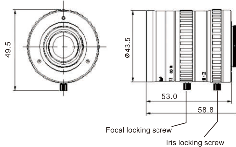
Unit: mm
